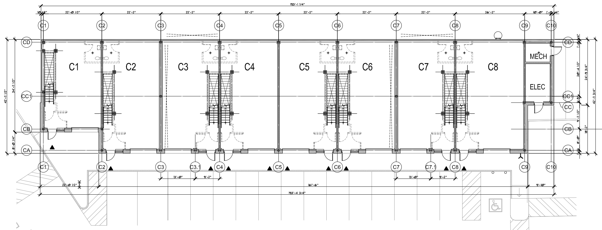
1 GROUND FLOOR PLAN - OVERVIEW SCALE: AS PER SCALE BAR
