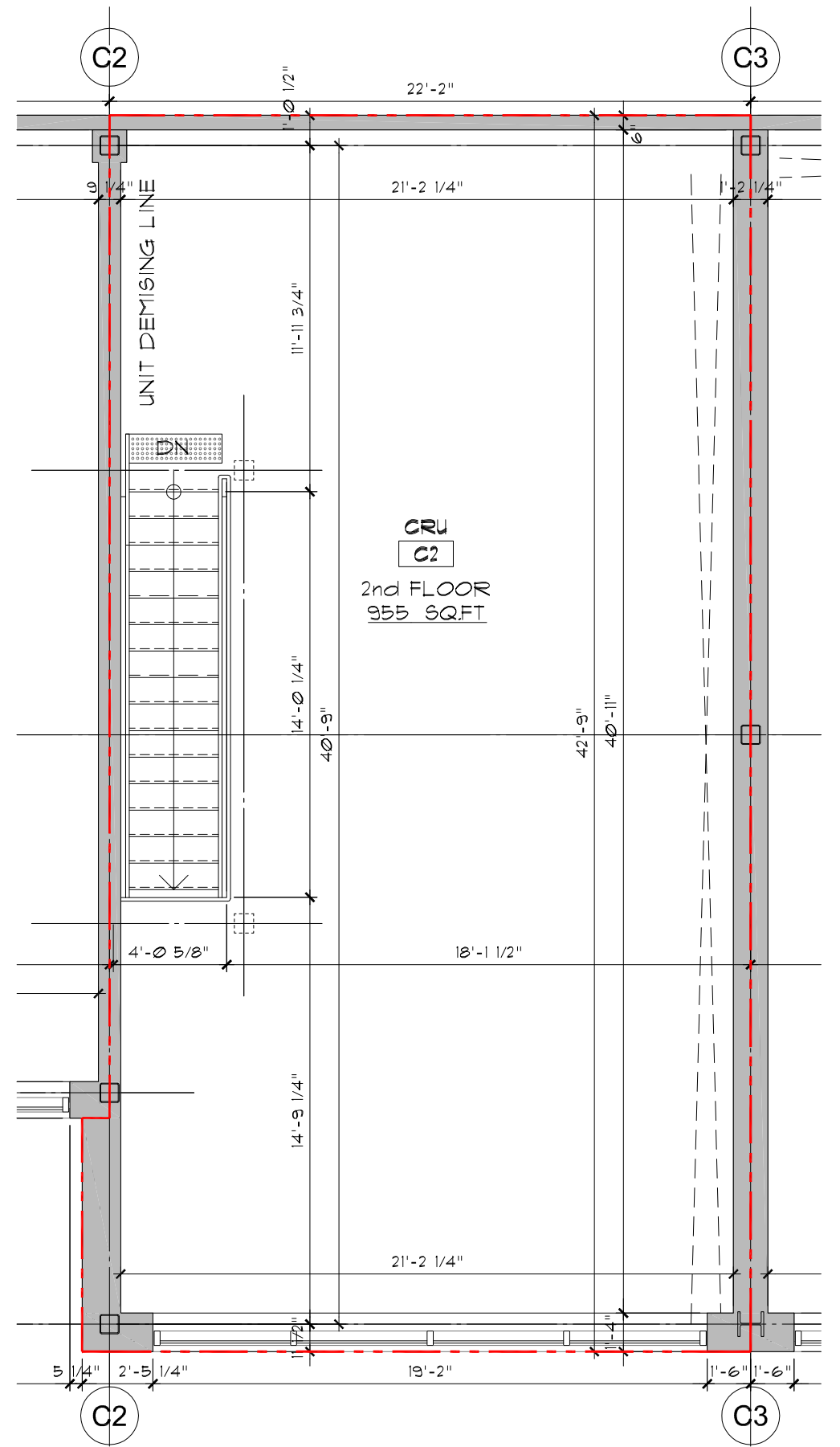
2 UNIT C2 - SECOND FLOOR SCALE: AS PER SCALE BAR
