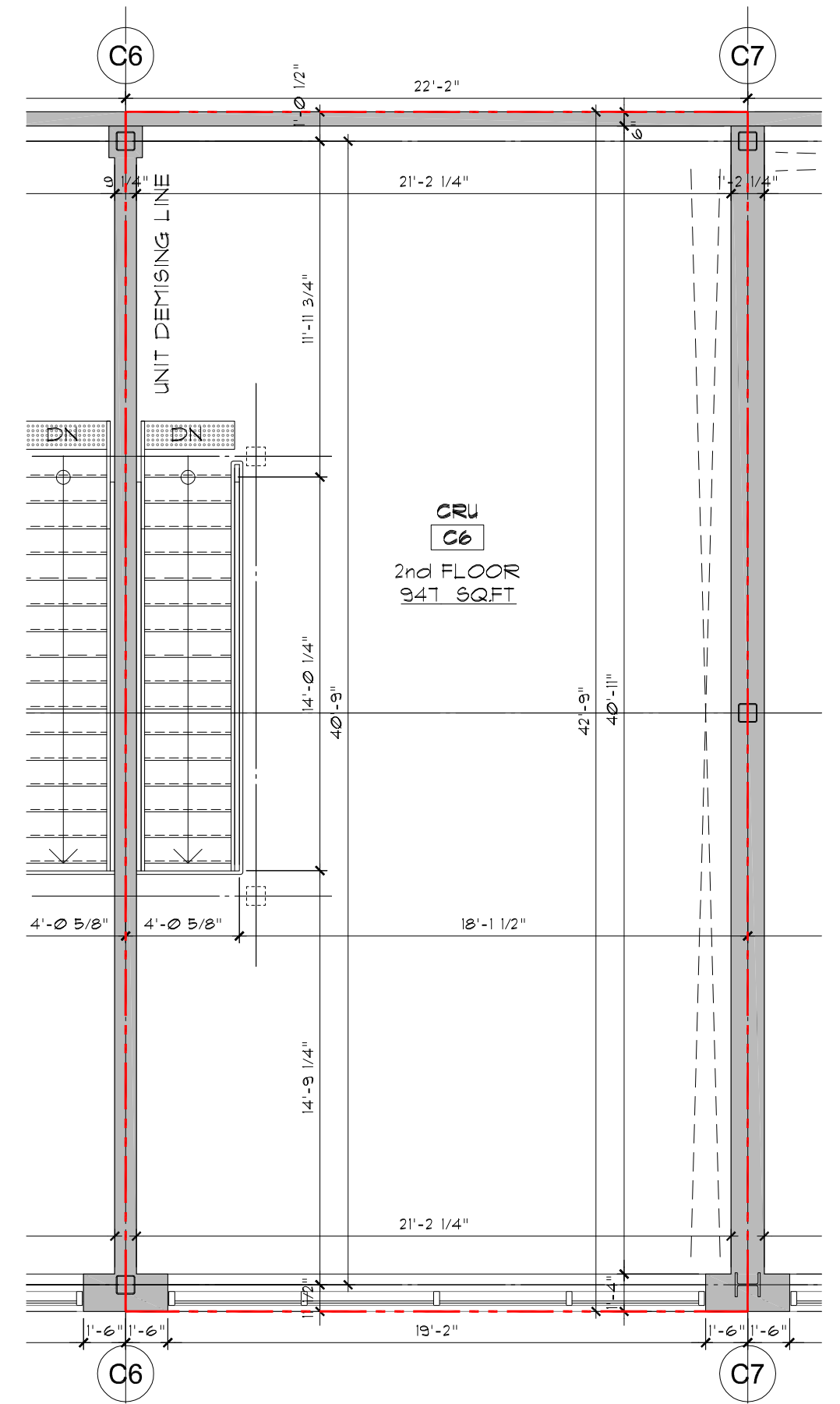
2 UNIT C6 - SECOND FLOOR SCALE: AS PER SCALE BAR
