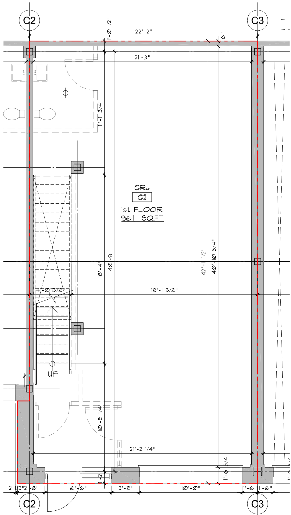
1 UNIT C2 - GROUND FLOOR SCALE: AS PER SCALE BAR
