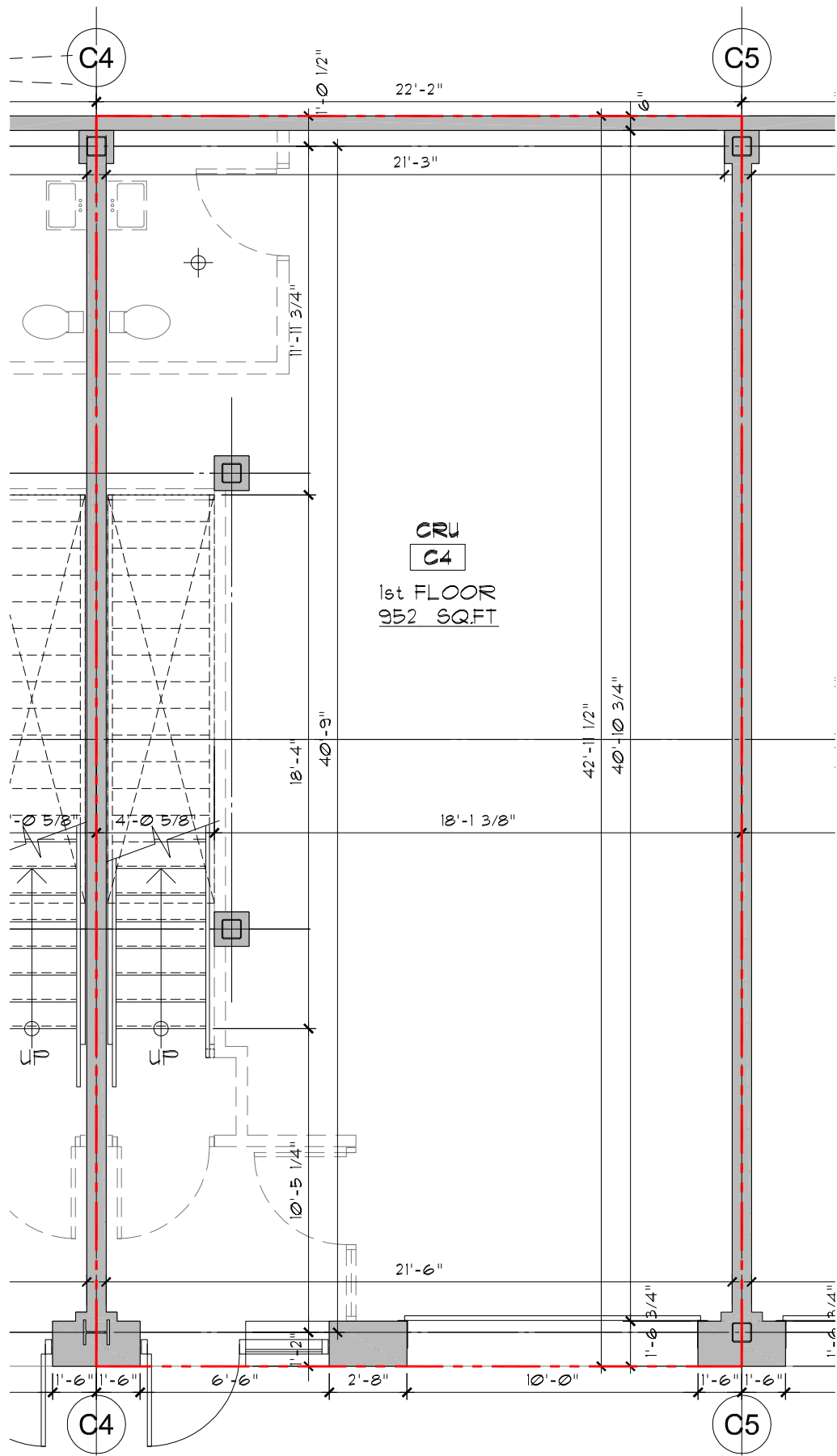
1 UNIT C4 - GROUND FLOOR SCALE: AS PER SCALE BAR
