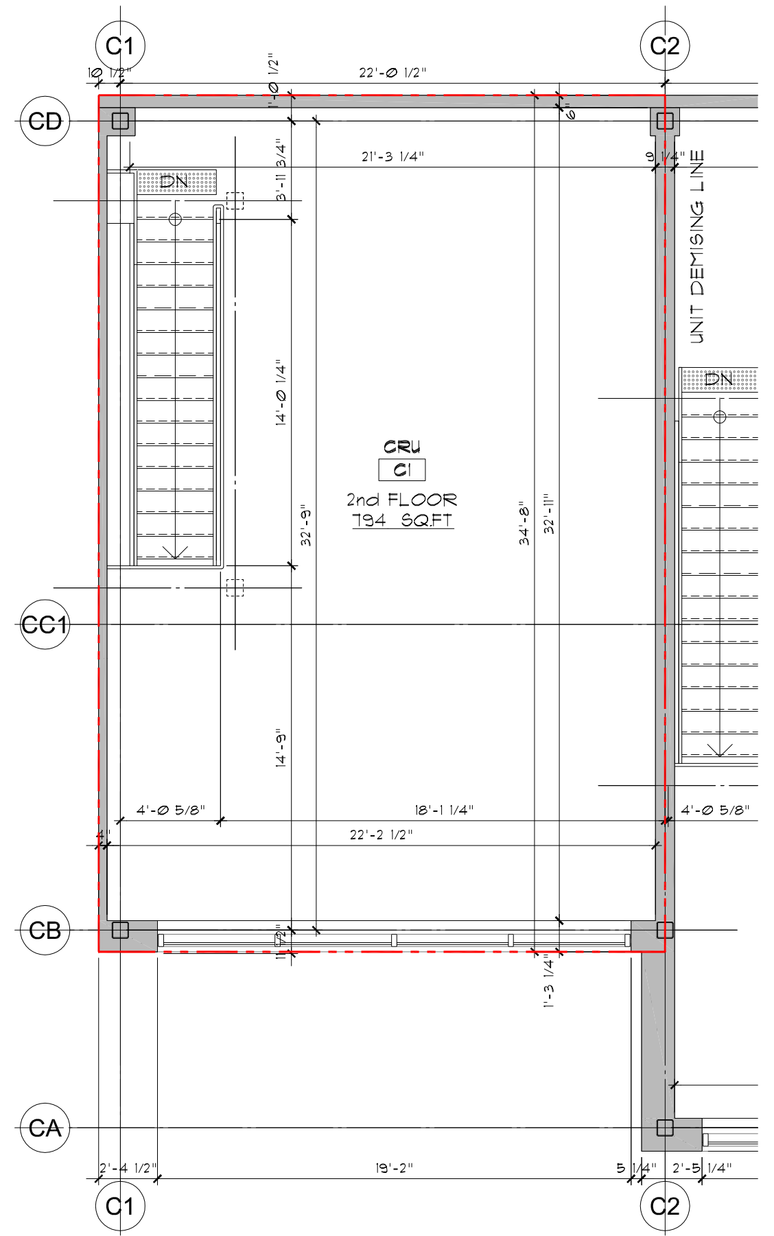
2 UNIT C1 - SECOND FLOOR SCALE: AS PER SCALE BAR
