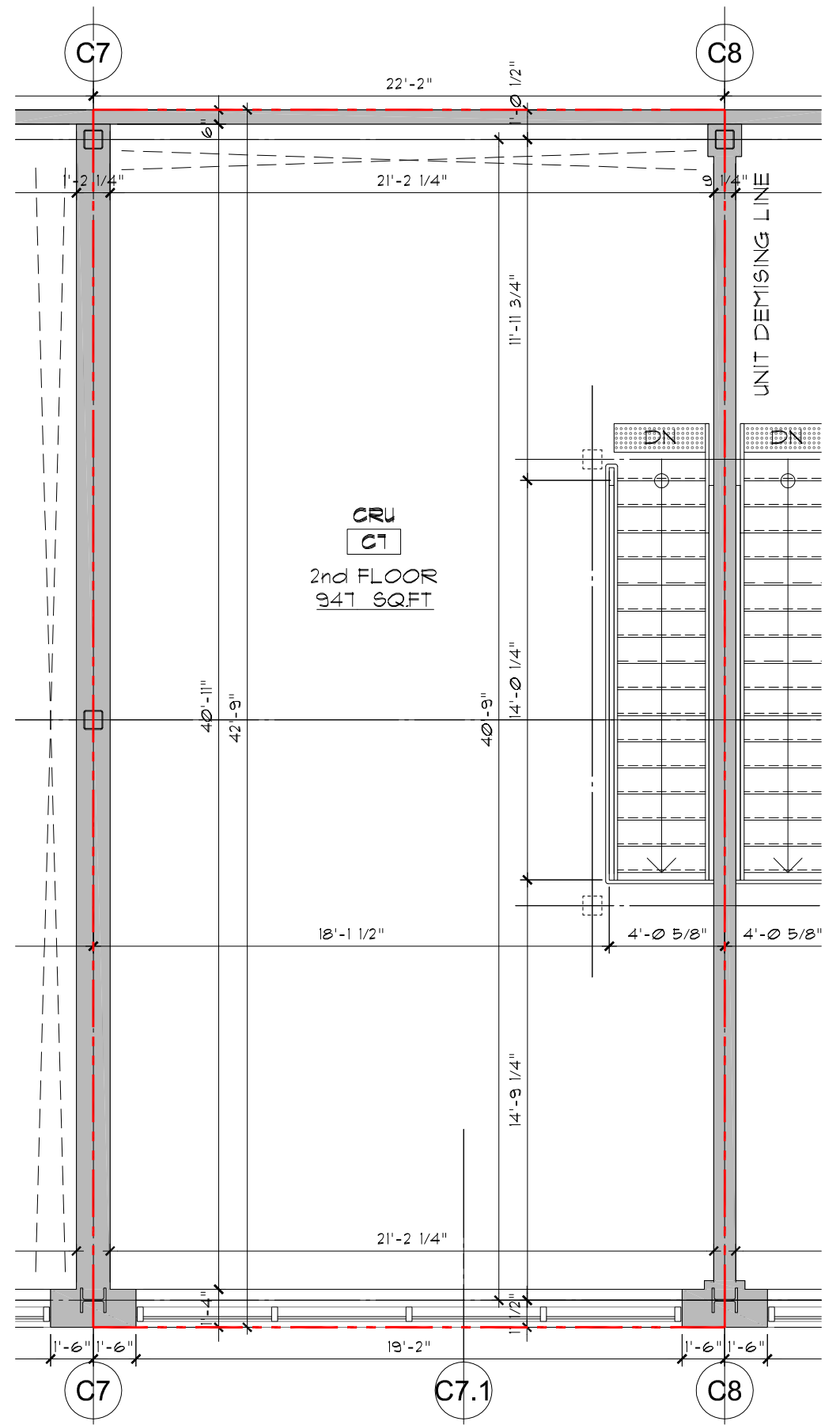
2 UNIT C7 - SECOND FLOOR SCALE: AS PER SCALE BAR
