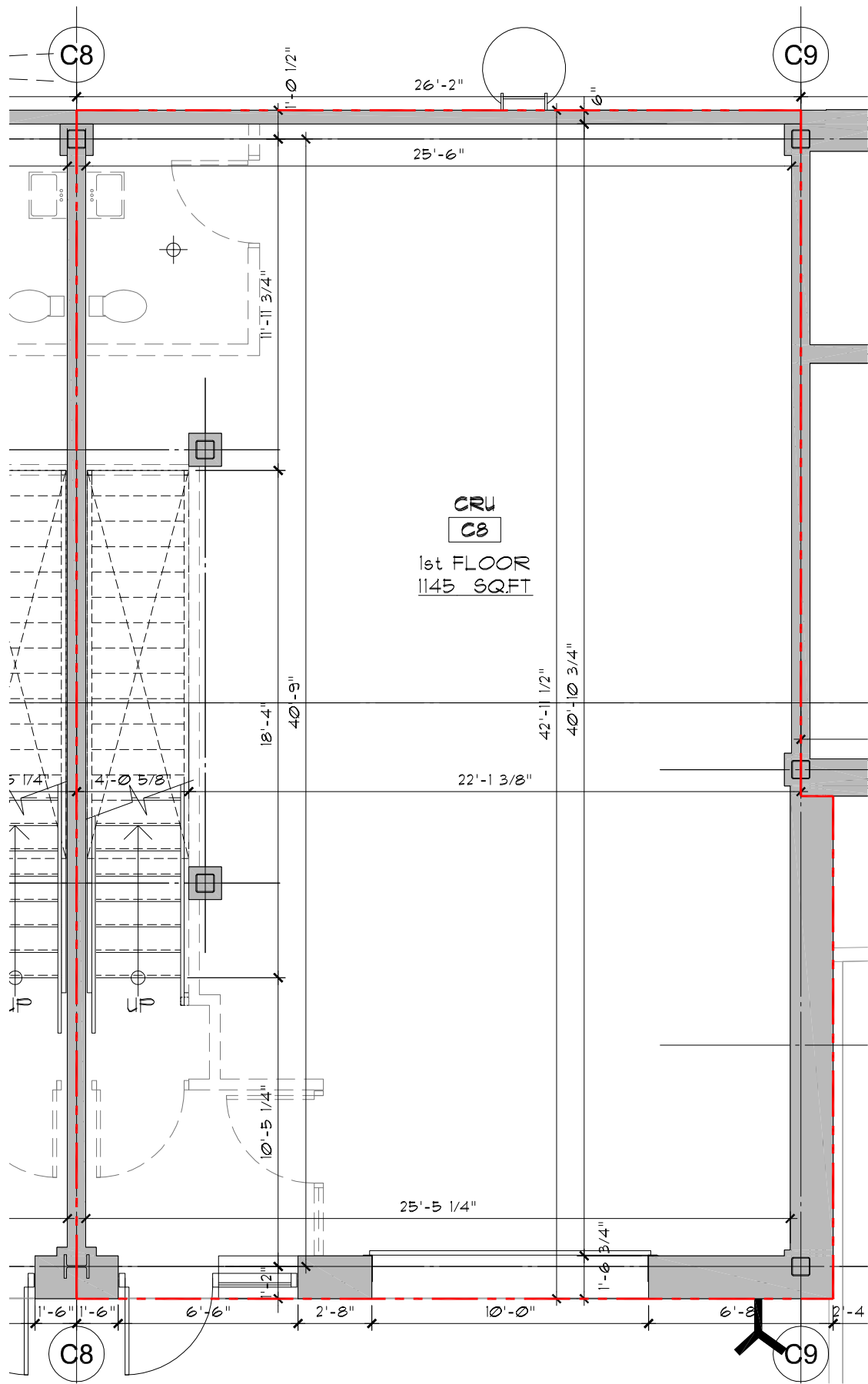
1 UNIT C8 - GROUND FLOOR SCALE: AS PER SCALE BAR
