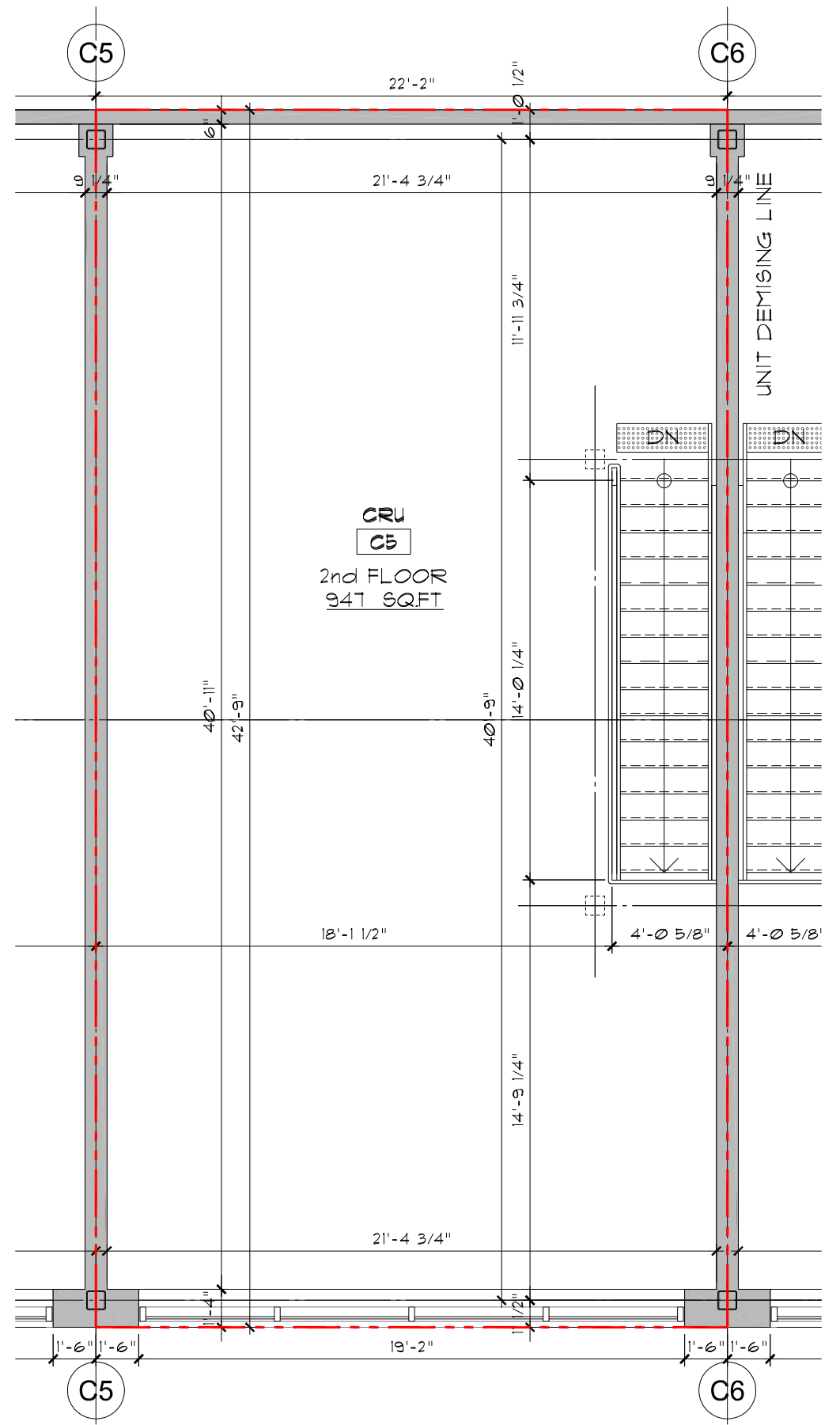
2 UNIT C5 - SECOND FLOOR SCALE: AS PER SCALE BAR
