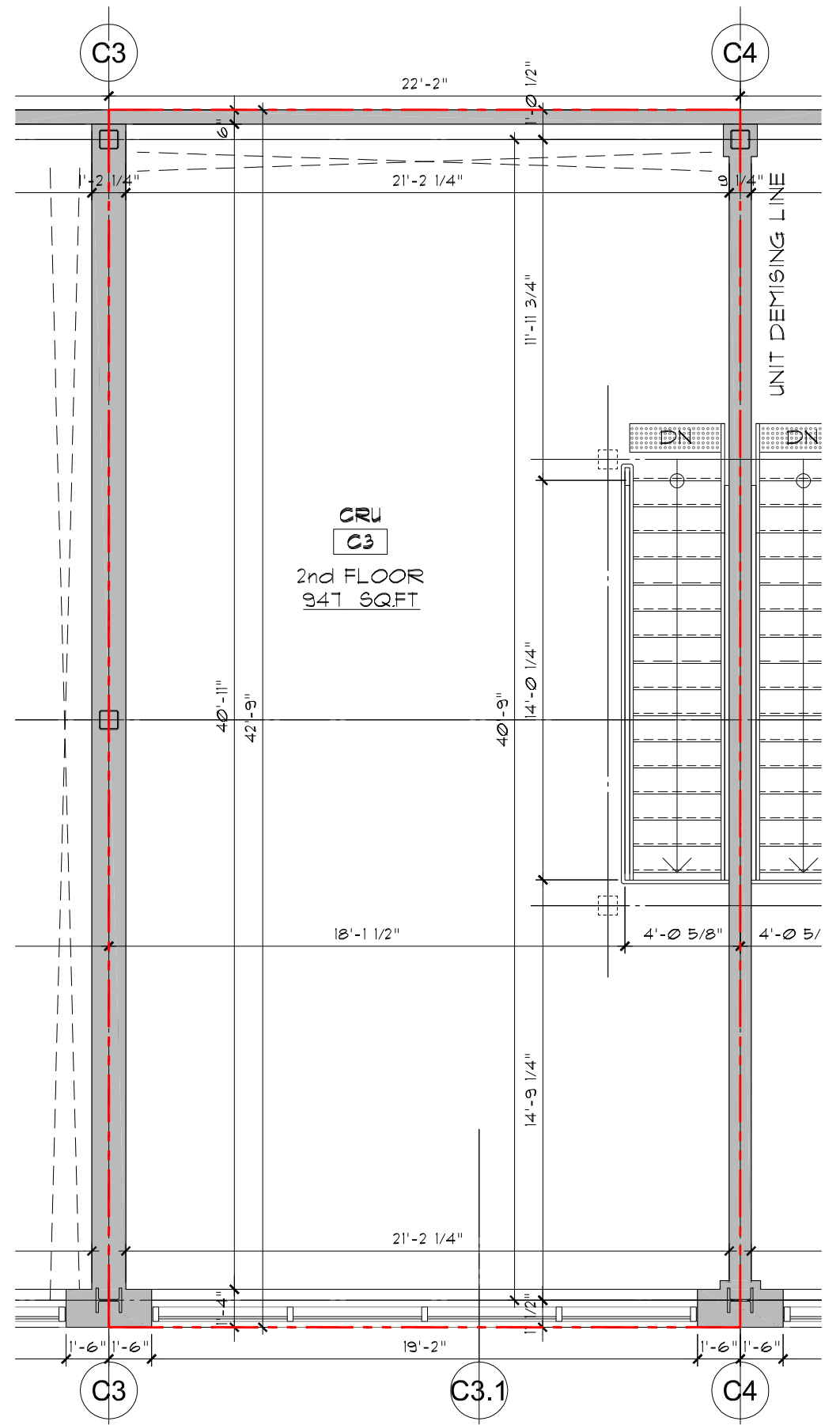
2 UNIT C3 - SECOND FLOOR SCALE: AS PER SCALE BAR
