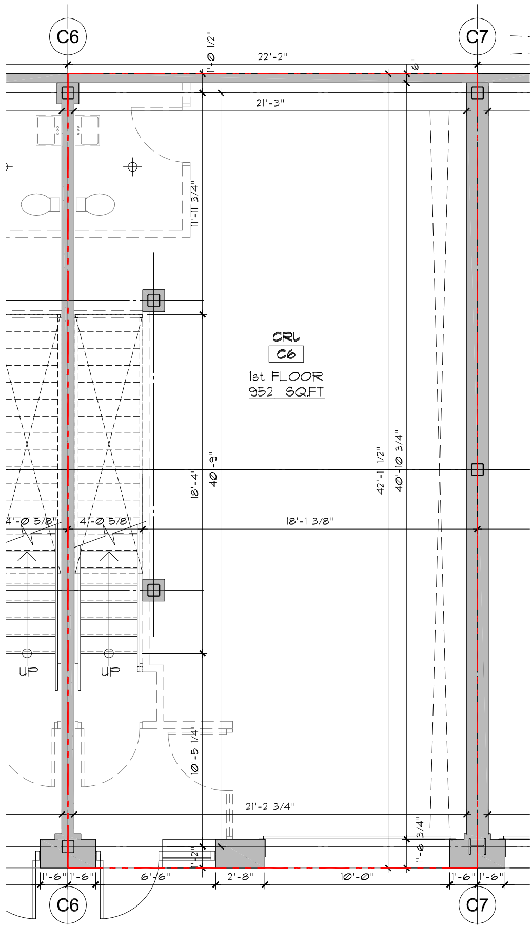
1 UNIT C6 - GROUND FLOOR SCALE: AS PER SCALE BAR
