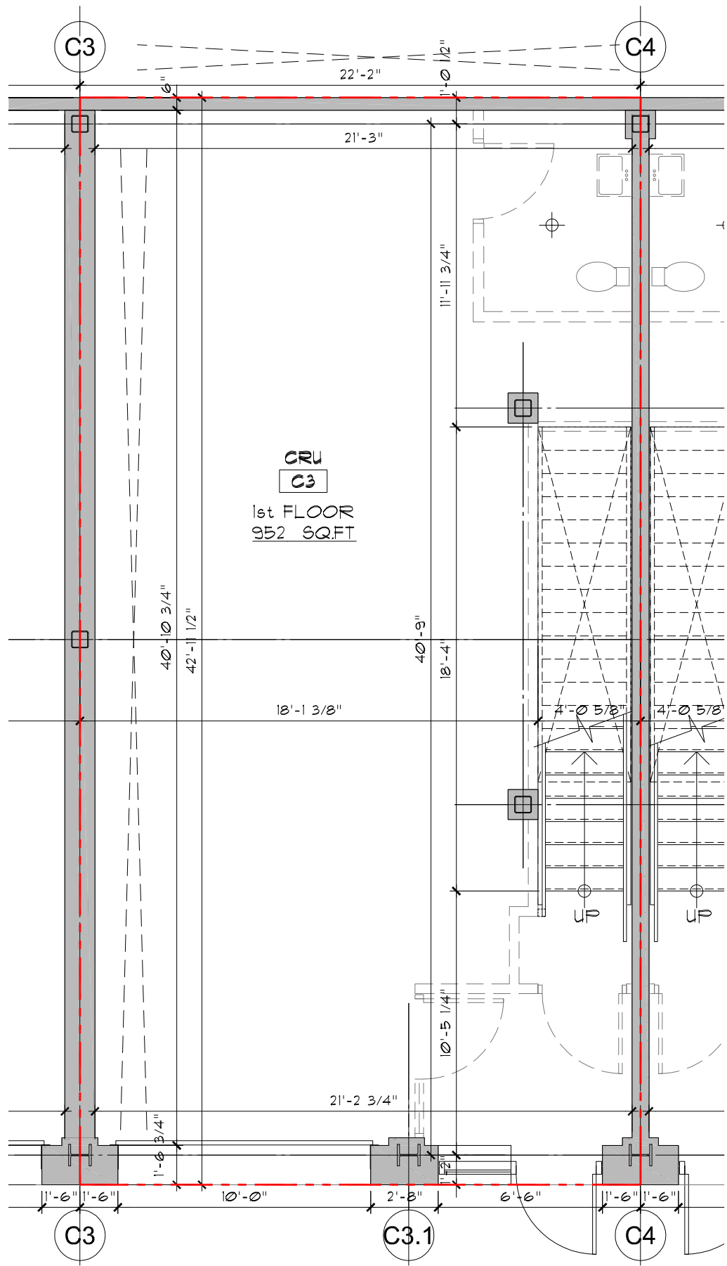
1 UNIT C3 - GROUND FLOOR SCALE: AS PER SCALE BAR
