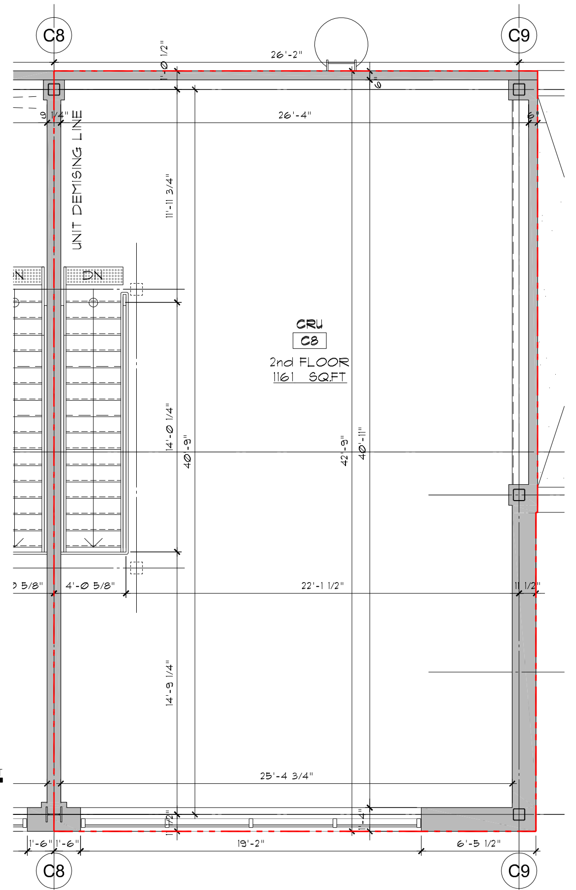
2 UNIT C8 - SECOND FLOOR SCALE: AS PER SCALE BAR
