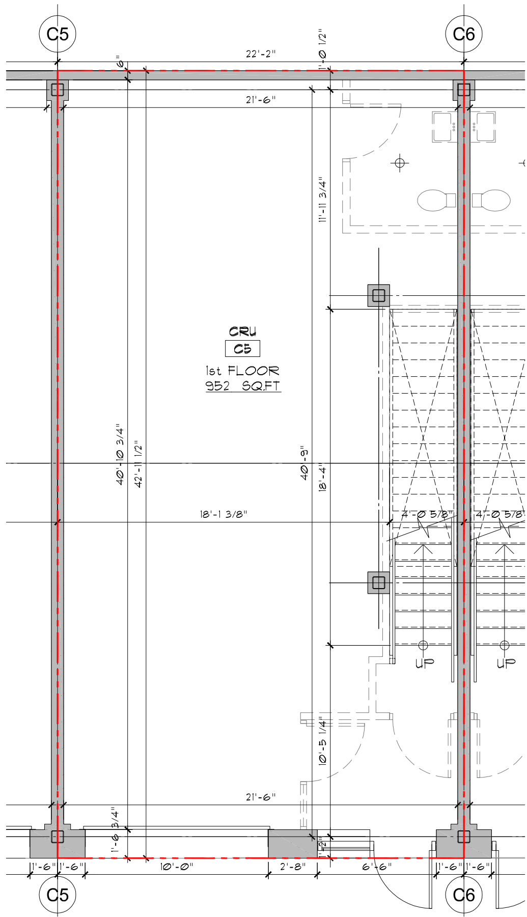
1 UNIT C5 - GROUND FLOOR SCALE: AS PER SCALE BAR
