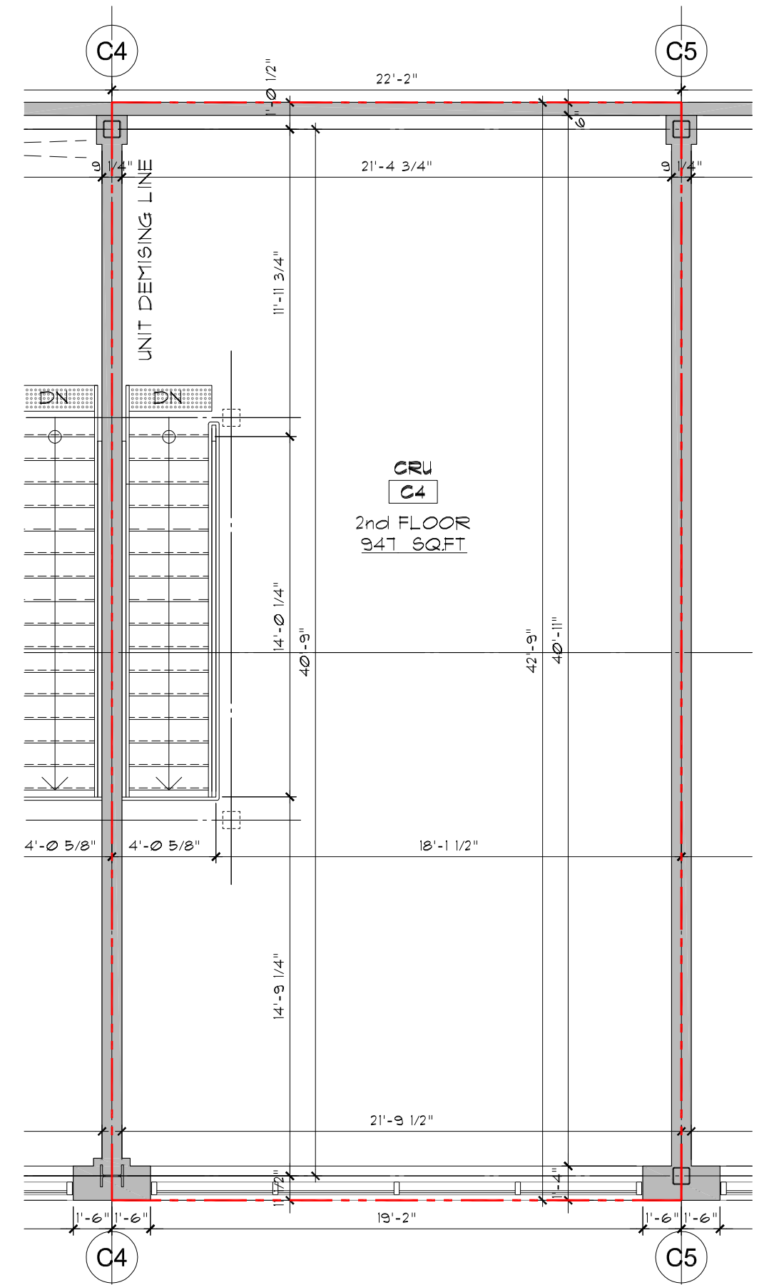
2 UNIT C4 - SECOND FLOOR SCALE: AS PER SCALE BAR
