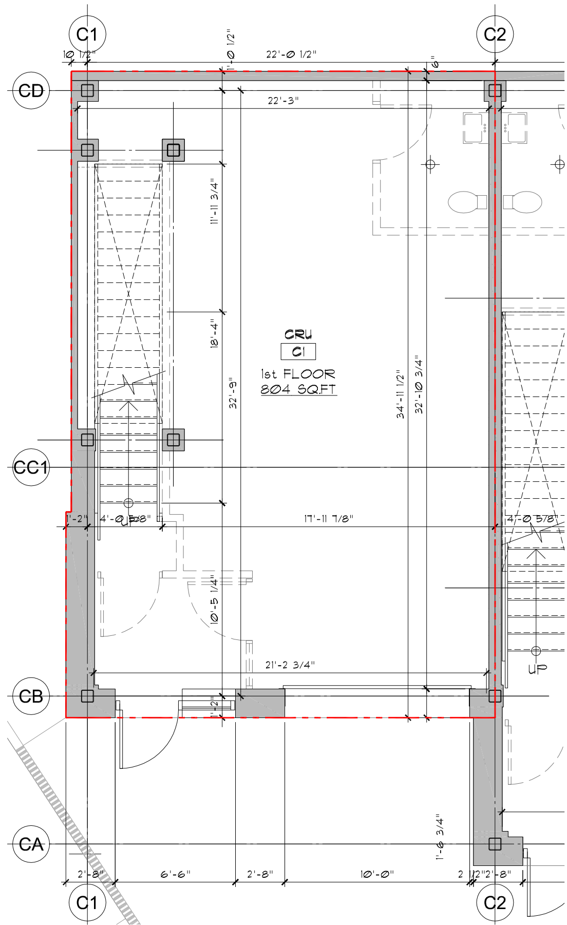
1 UNIT C1 - GROUND FLOOR SCALE: AS PER SCALE BAR
