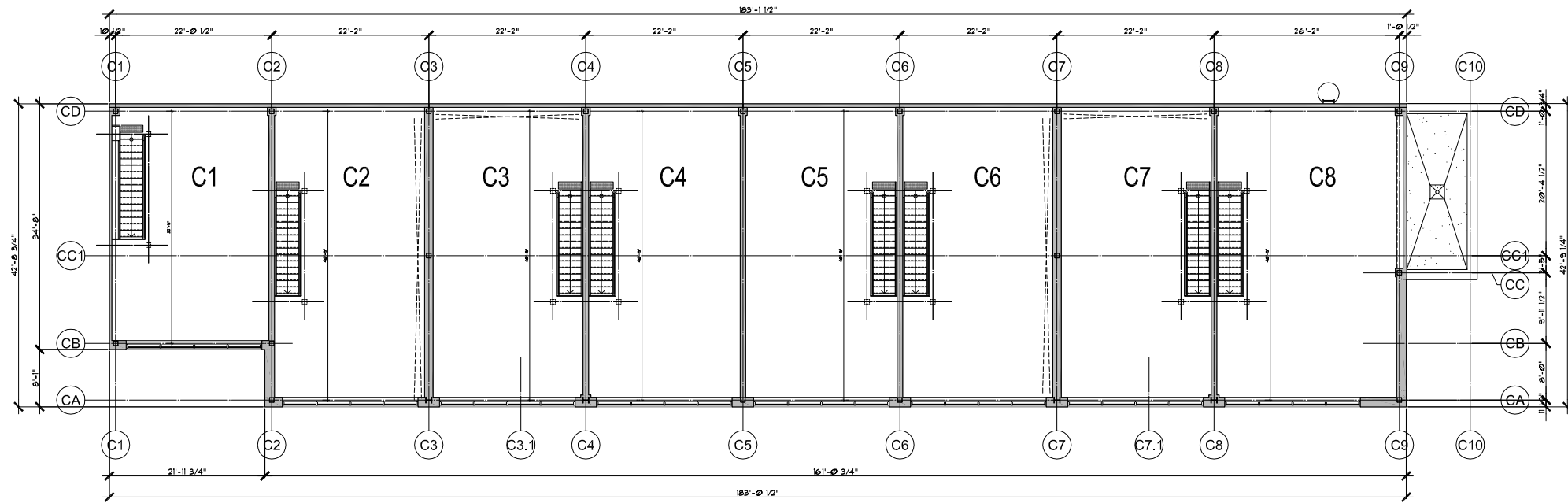
2 SECOND FLOOR PLAN - OVERVIEW SCALE: AS PER SCALE BAR
