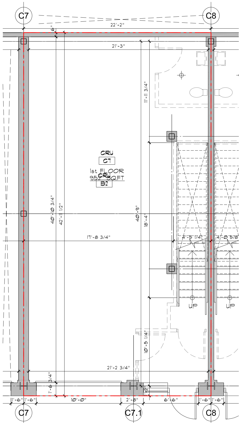
1 UNIT C7 - GROUND FLOOR SCALE: AS PER SCALE BAR
