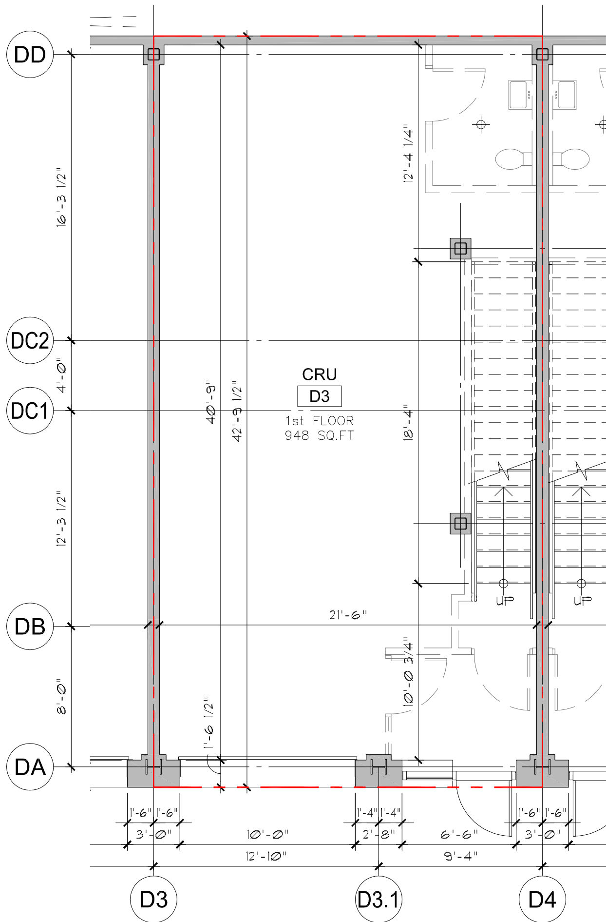
1 UNIT D3 - GROUND FLOOR SCALE: AS PER SCALE BAR
