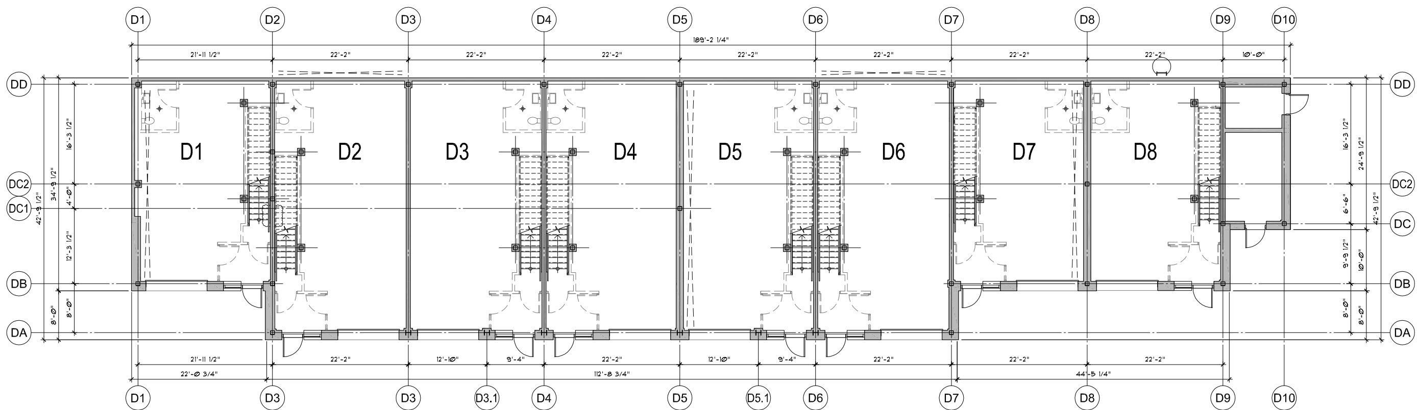
1 GROUND FLOOR PLAN - OVERVIEW SCALE: AS PER SCALE BAR
