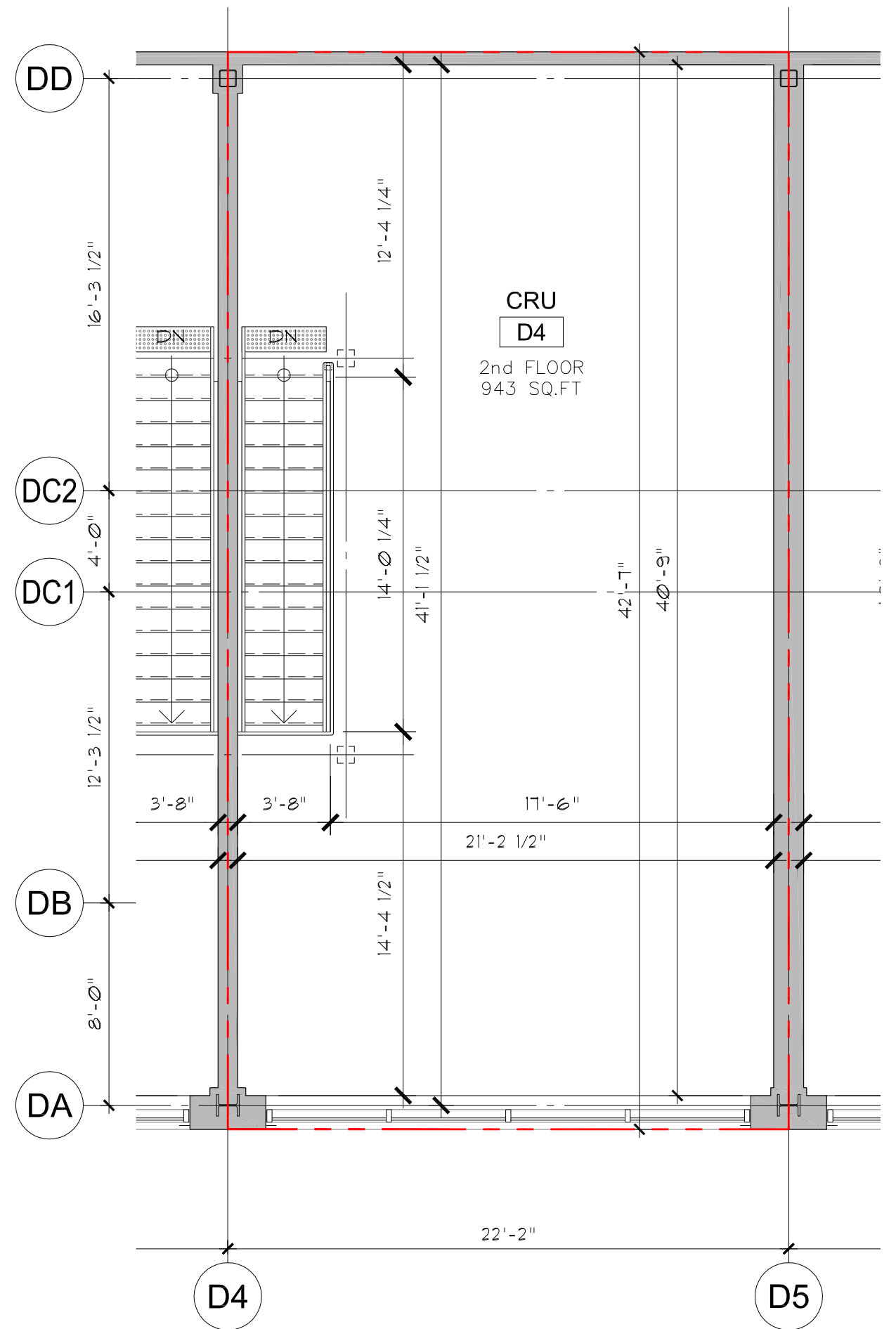
2 UNIT D4 - SECOND FLOOR SCALE: AS PER SCALE BAR
