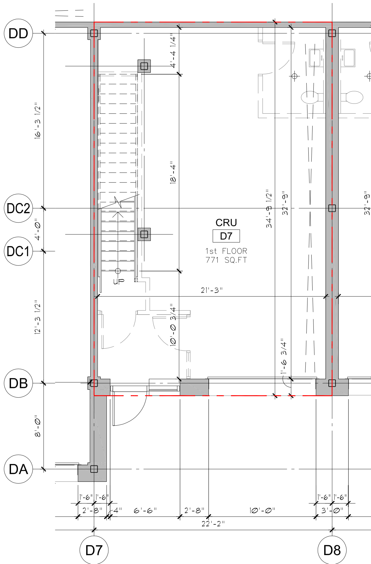
1 UNIT D7 - GROUND FLOOR SCALE: AS PER SCALE BAR
