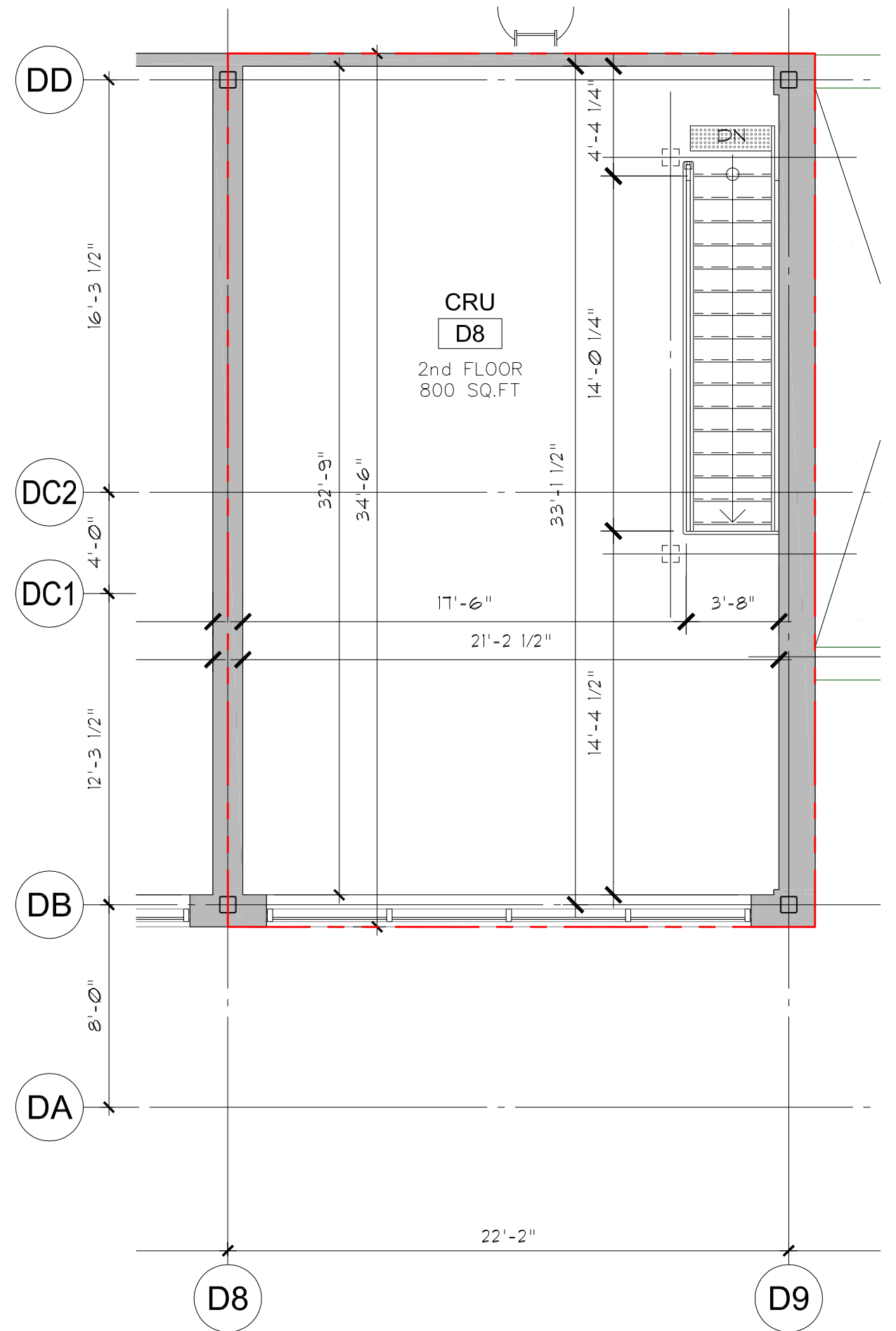
2 UNIT D8 - SECOND FLOOR SCALE: AS PER SCALE BAR
