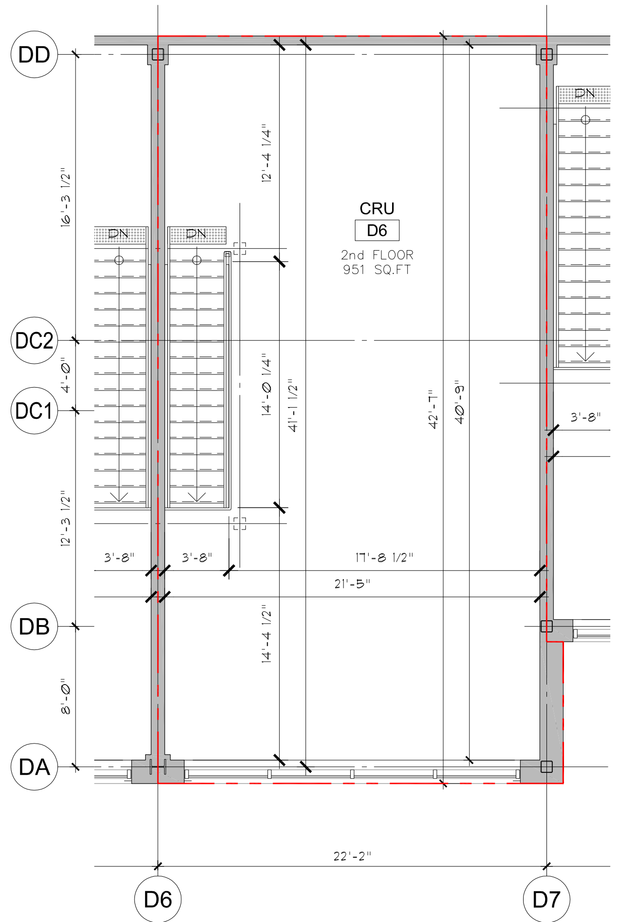
2 UNIT D6 - SECOND FLOOR SCALE: AS PER SCALE BAR
