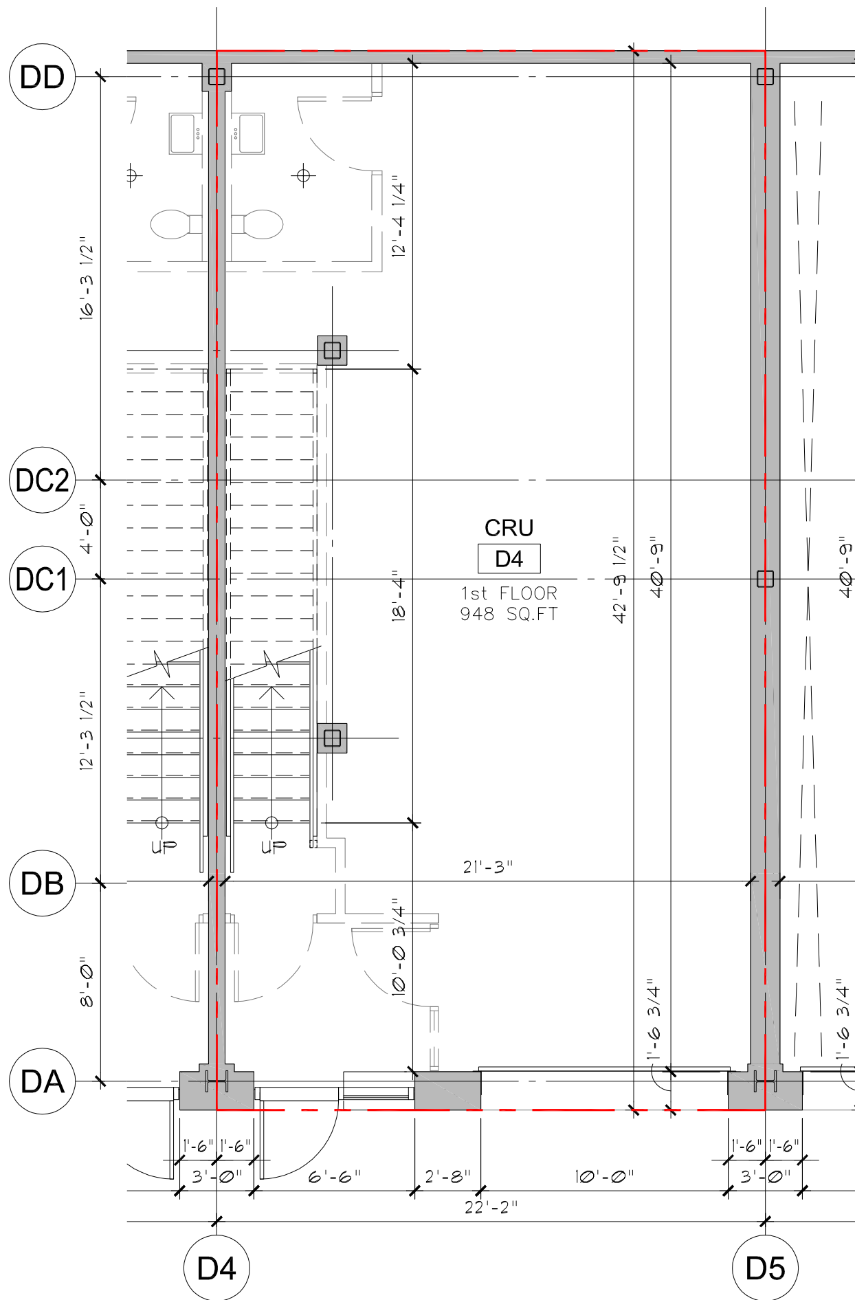
1 UNIT D4 - GROUND FLOOR SCALE: AS PER SCALE BAR
