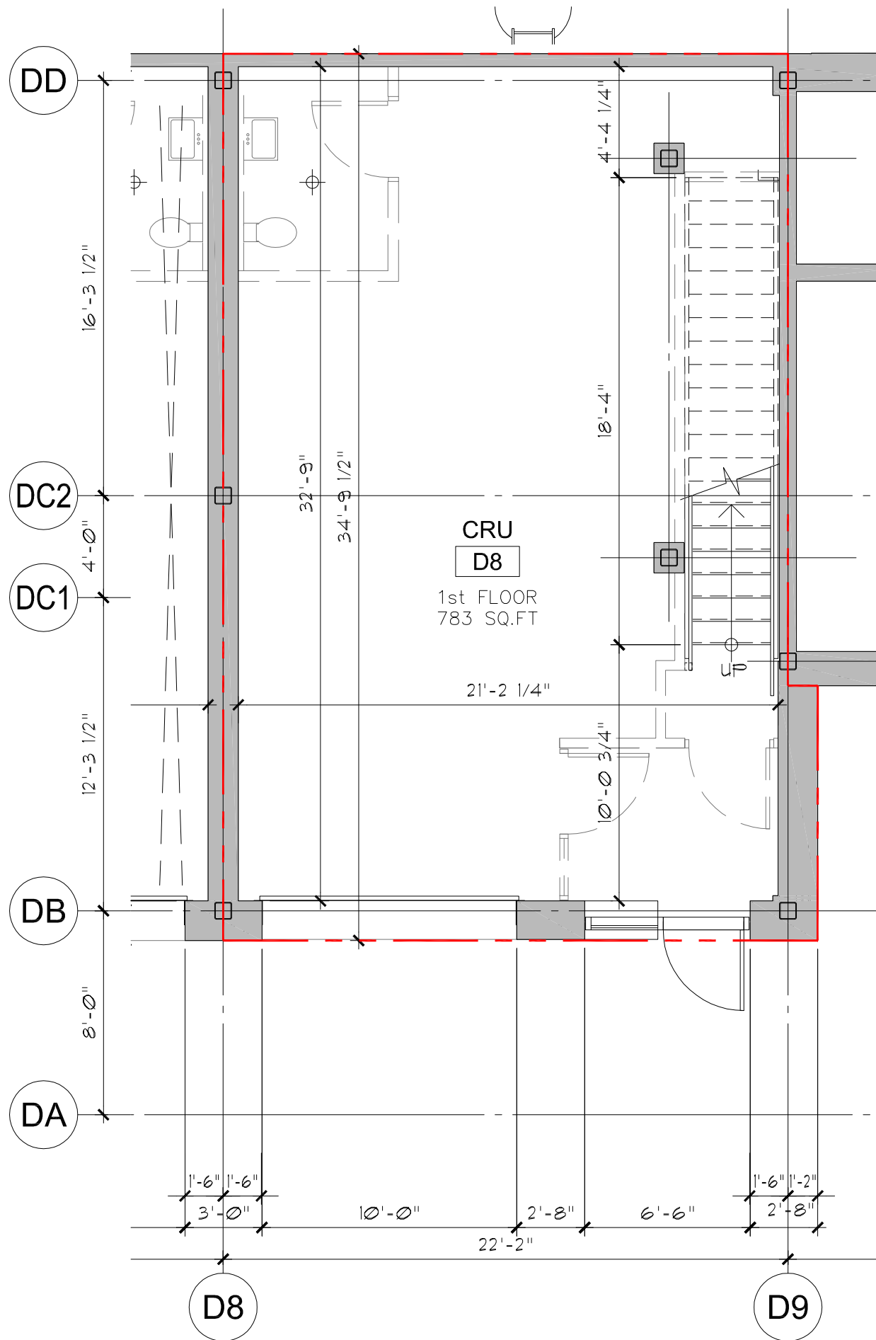
1 UNIT D8 - GROUND FLOOR SCALE: AS PER SCALE BAR
