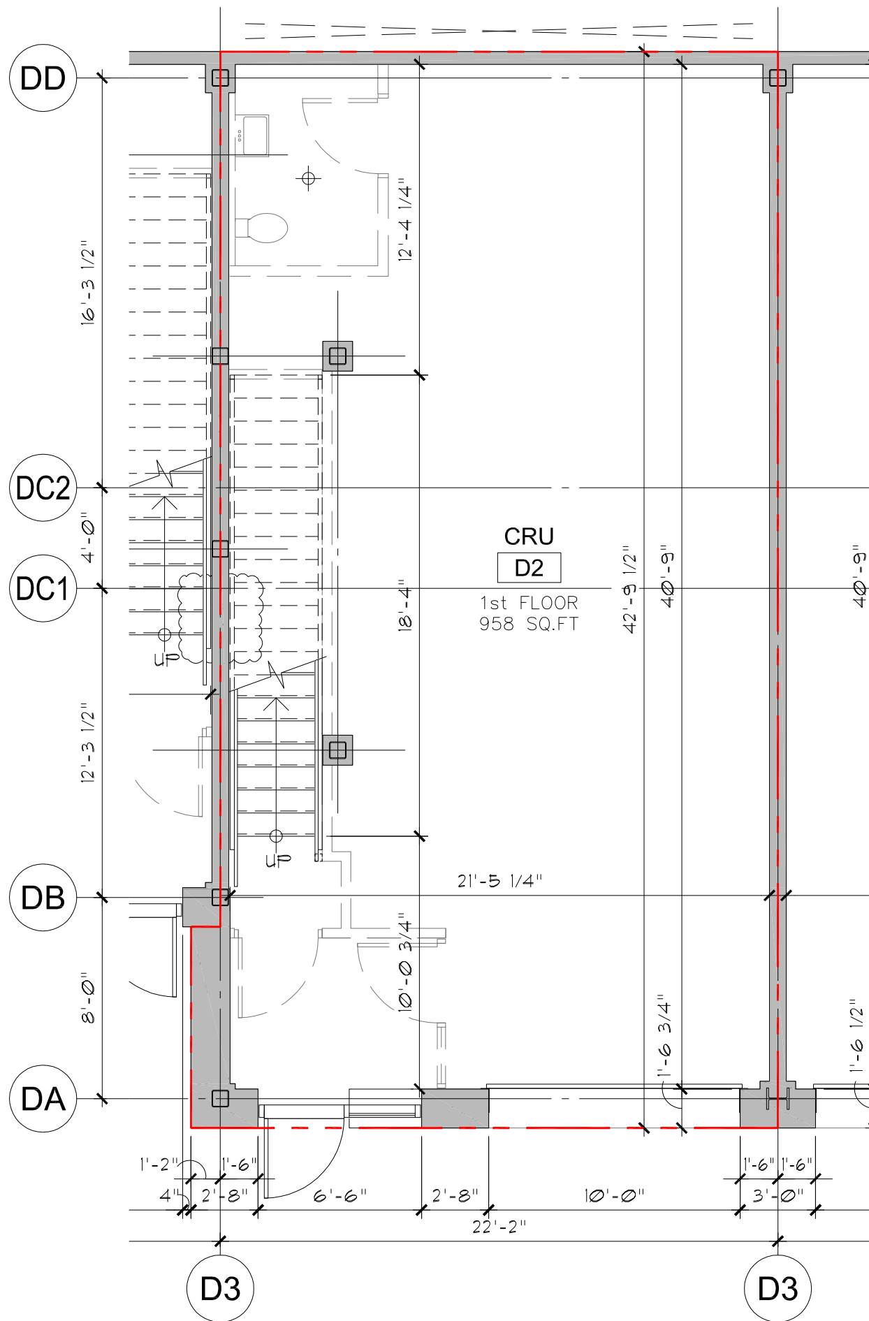
1 UNIT D2 - GROUND FLOOR SCALE: AS PER SCALE BAR
