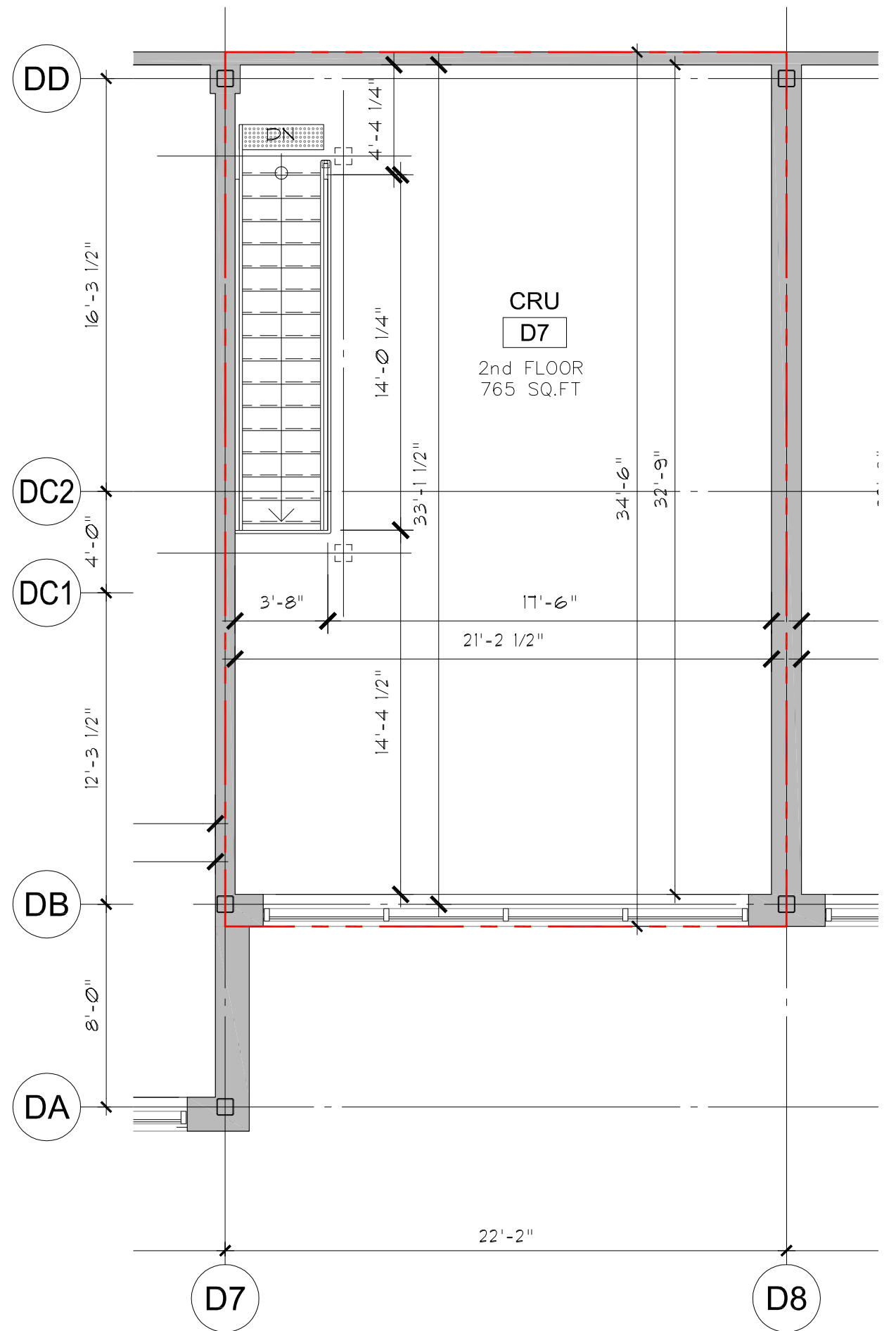
2 UNIT D7 - SECOND FLOOR SCALE: AS PER SCALE BAR
