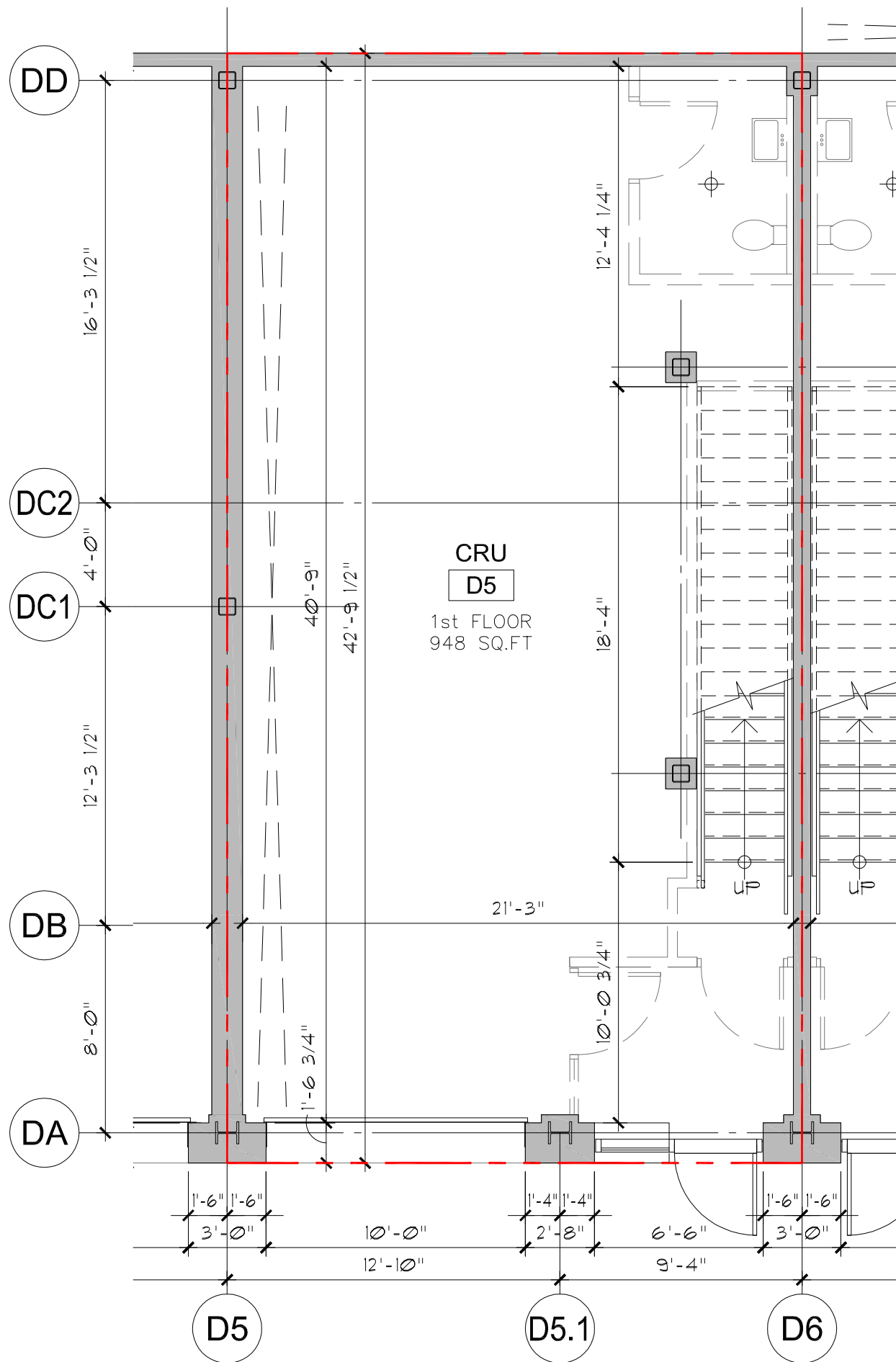
1 UNIT D5 - GROUND FLOOR SCALE: AS PER SCALE BAR
