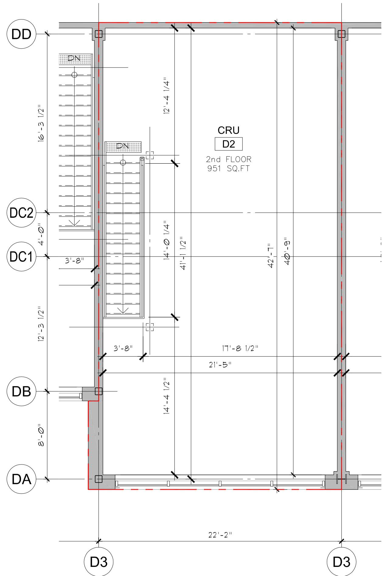
2 UNIT D2 - SECOND FLOOR SCALE: AS PER SCALE BAR
