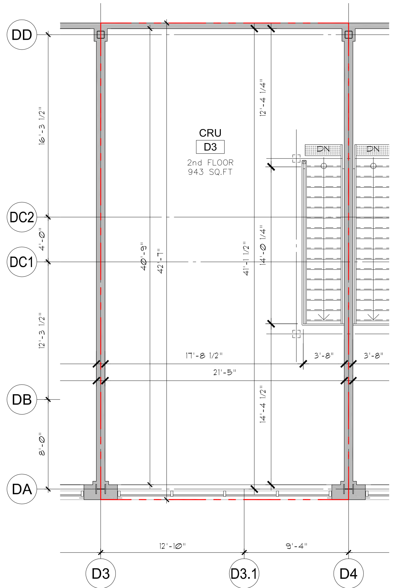
2 UNIT D3 - SECOND FLOOR SCALE: AS PER SCALE BAR
