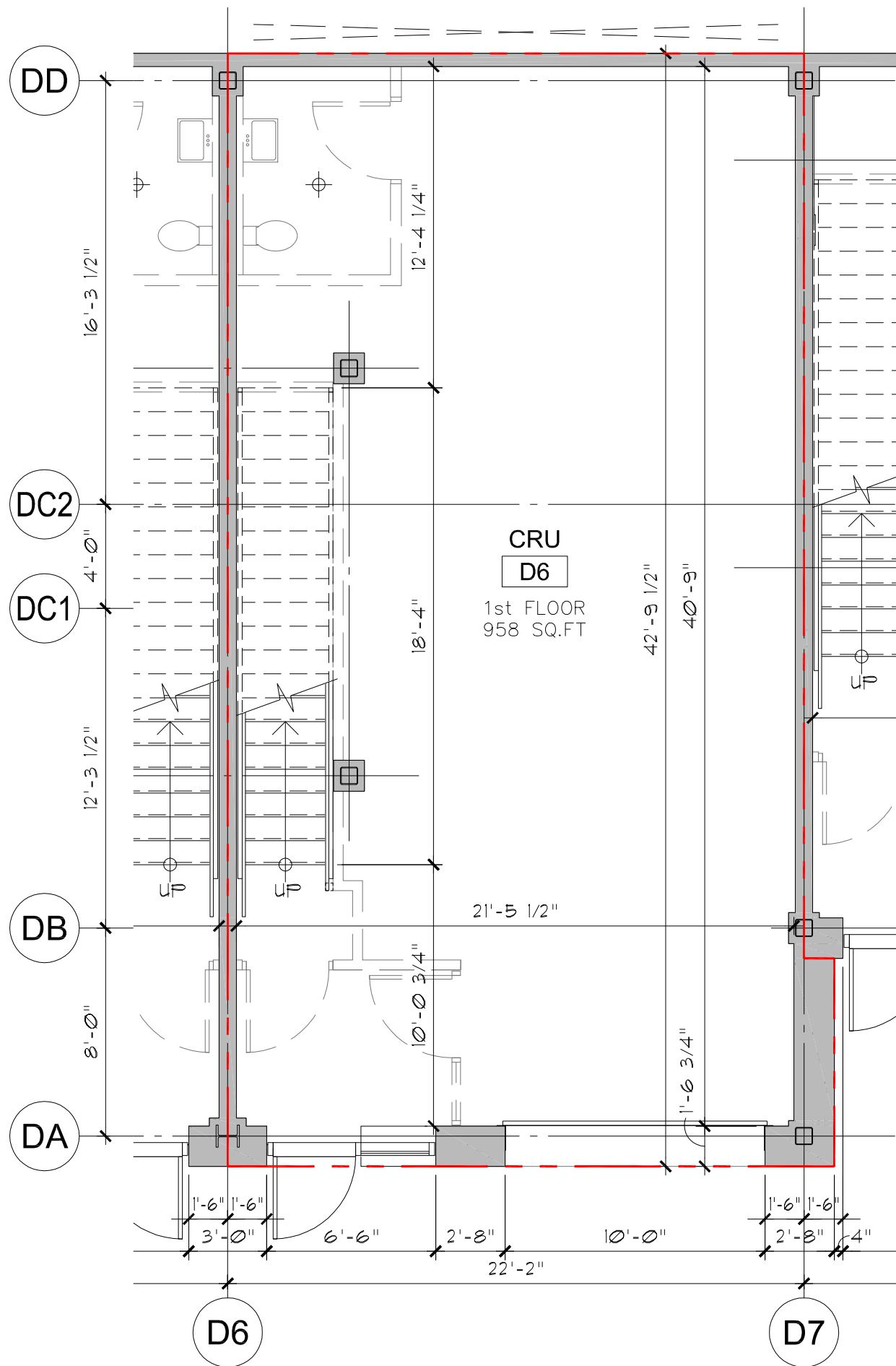
1 UNIT D6 - GROUND FLOOR SCALE: AS PER SCALE BAR
