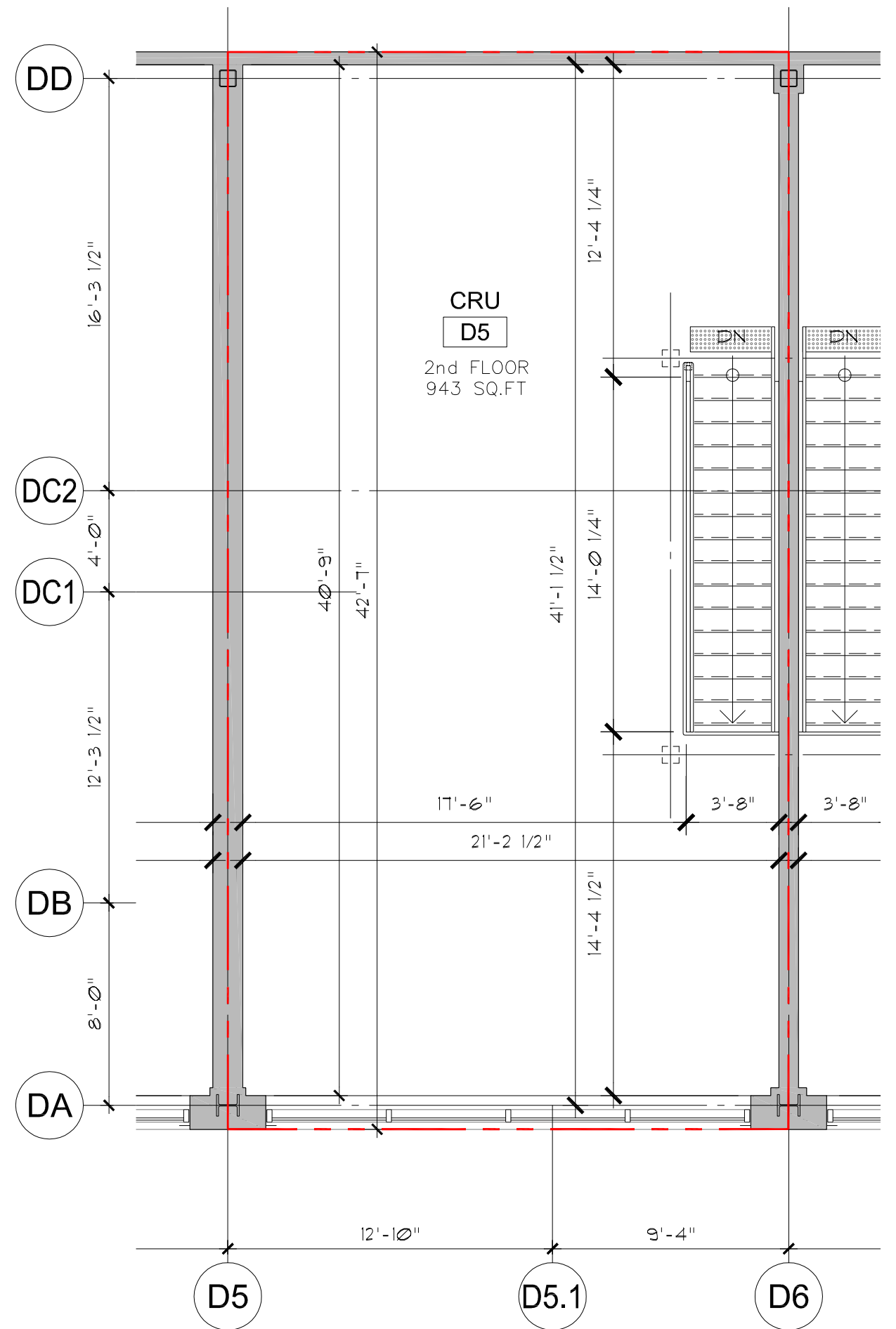
2 UNIT D5 - SECOND FLOOR SCALE: AS PER SCALE BAR
